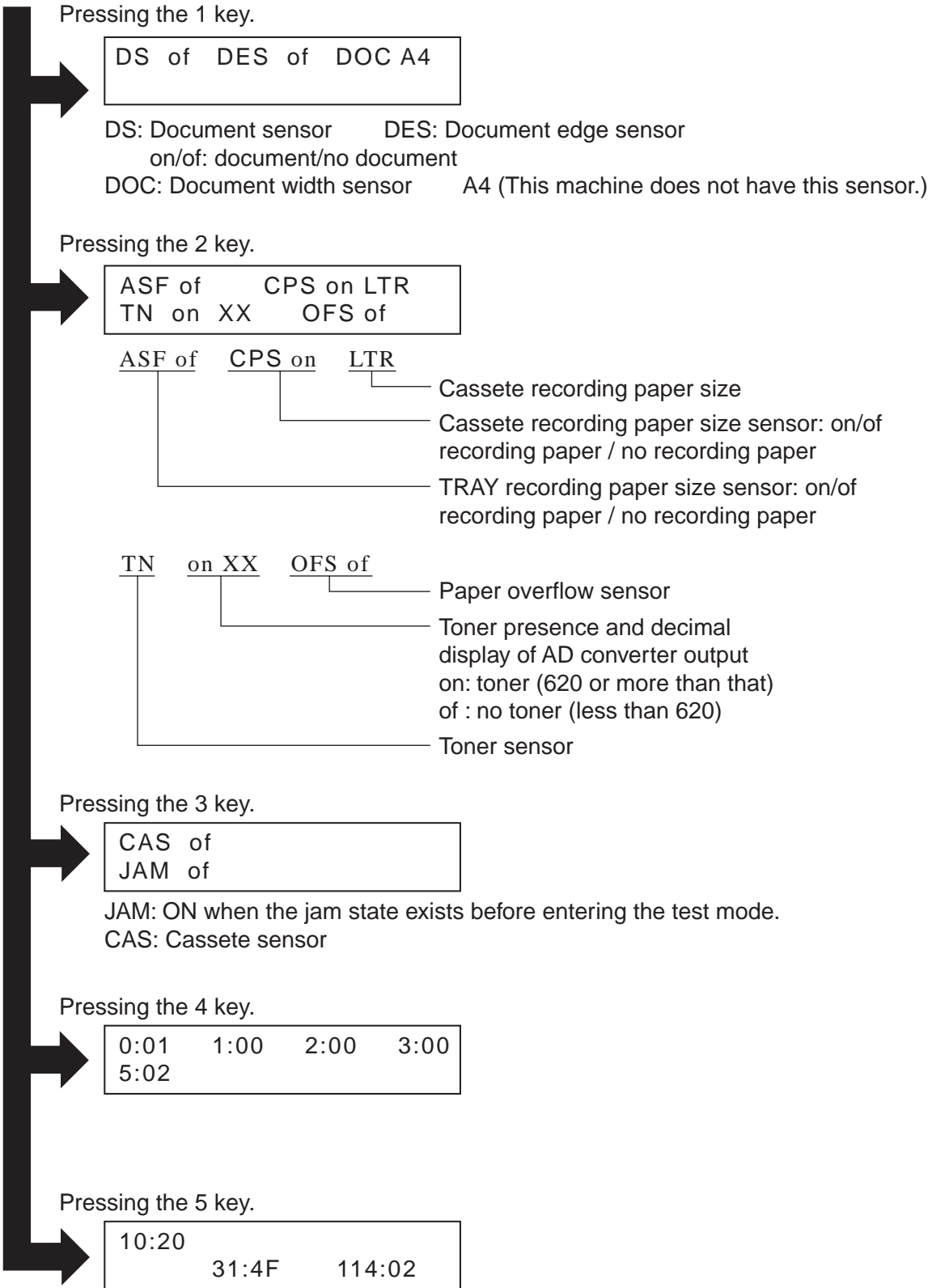
Figure 3-22 Sensor Tests
