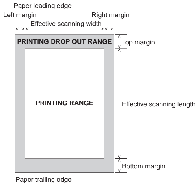
Figure 1-2 Printing Range
