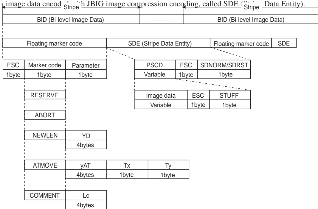
Figure 2-27 BID Construction Diagram
